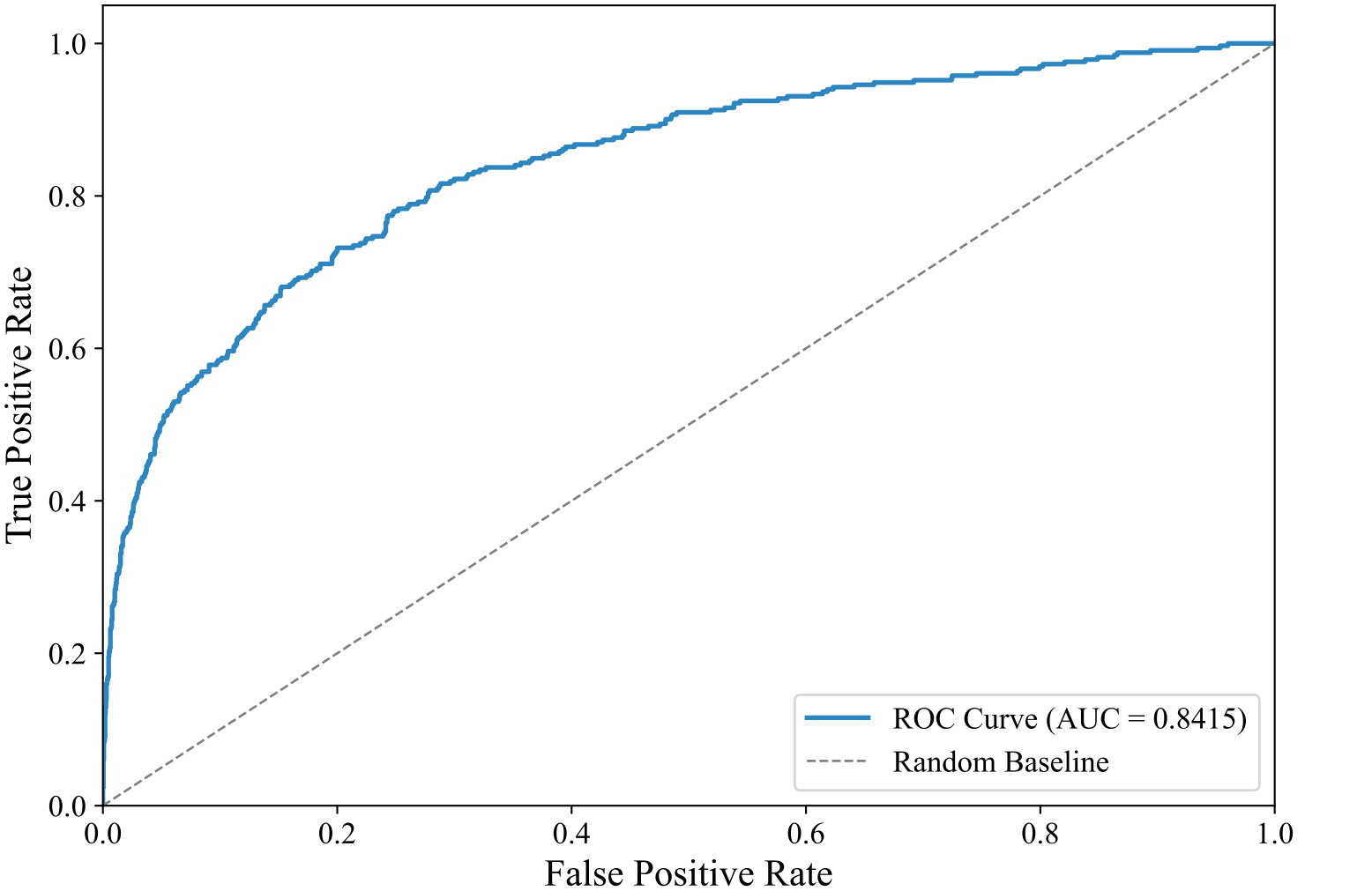
ROC Curve — GERMAN_MANUAL (upskyy/bge-m3-korean, LightGBM)
