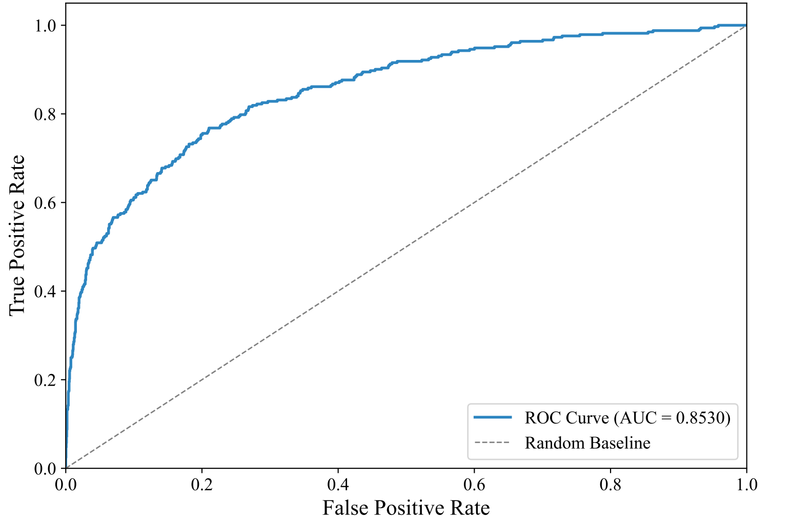
ROC Curve — GERMAN_MANUAL (upskyy/bge-m3-korean, XGBoost_Optimized)
