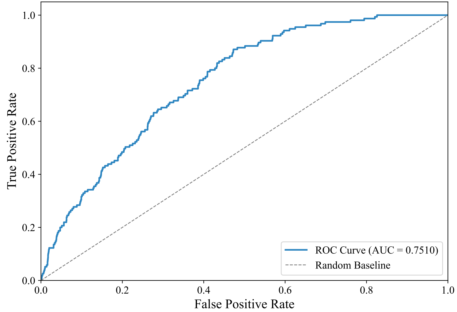
ROC Curve — SWEDISH_MANUAL (paraphrase-multilingual-MiniLM-L12-v2, Random_Forest)
