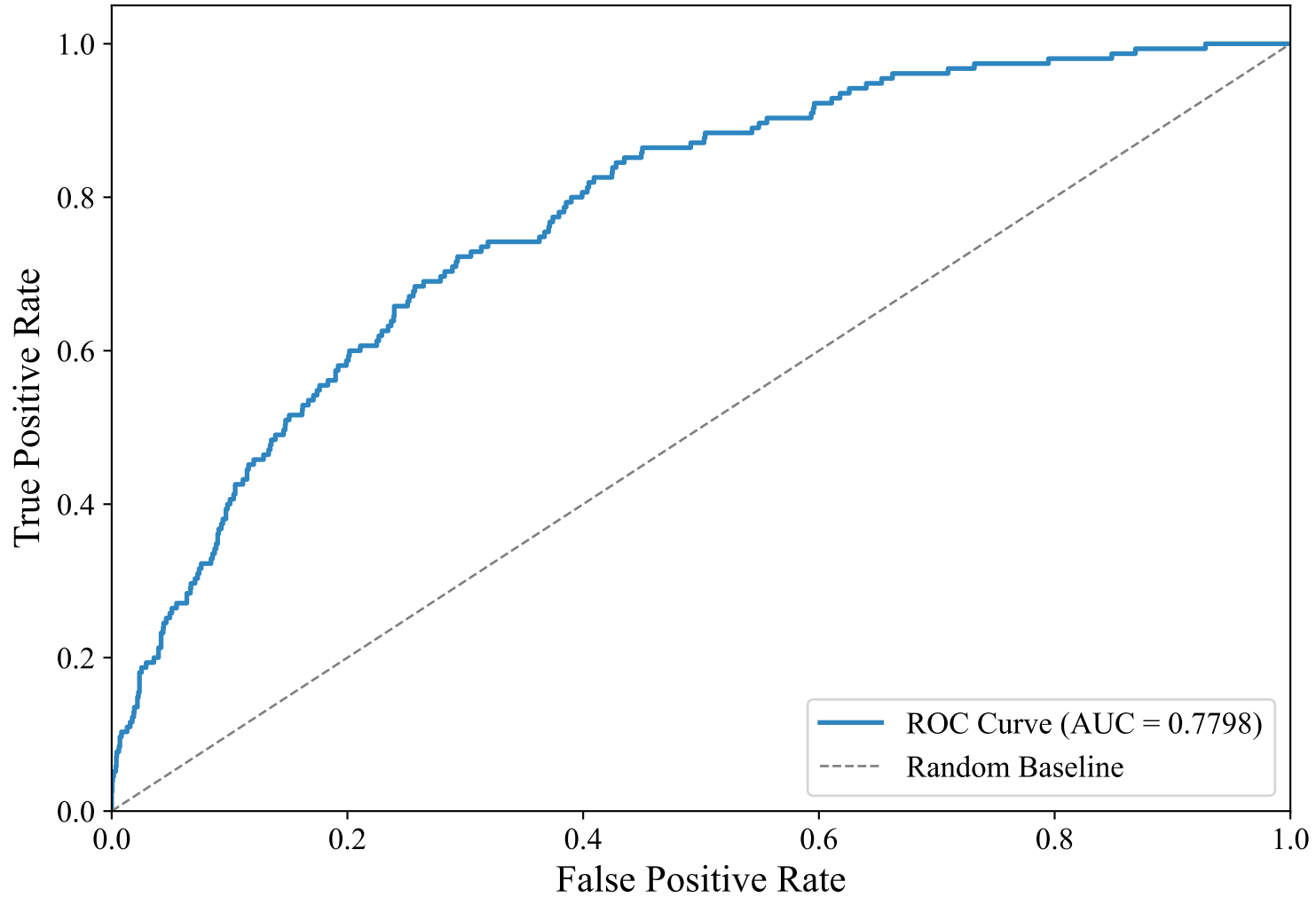
ROC Curve — SWEDISH_MANUAL (paraphrase-multilingual-mpnet-base-v2, XGBoost_Optimized)
