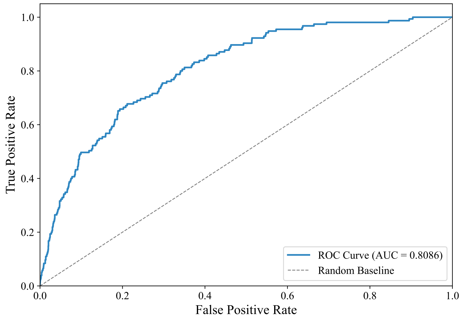
ROC Curve — SWEDISH_MANUAL (snowflake-arctic-embed-l-v2.0, XGBoost_Optimized)
