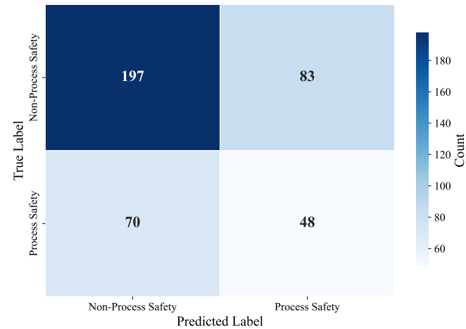
(f) xlnet-base-cased.
