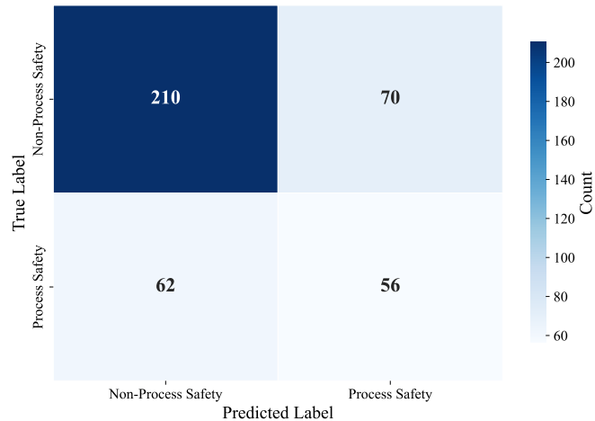
(a) bert-base-cased.
