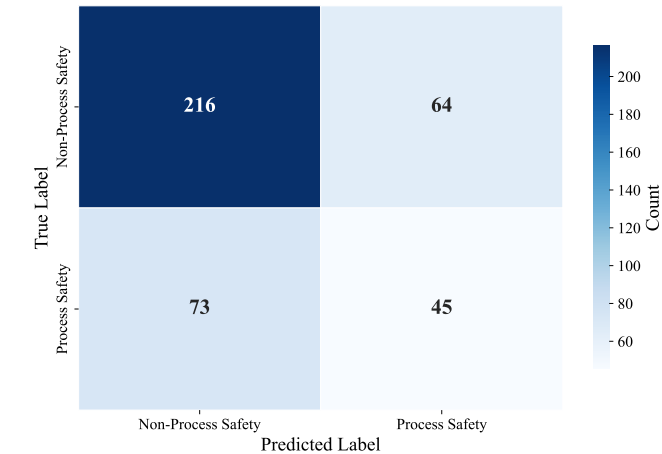
(c) distilbert-base-cased.
