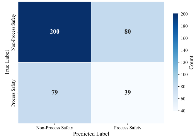
(b) bert-large-cased.
