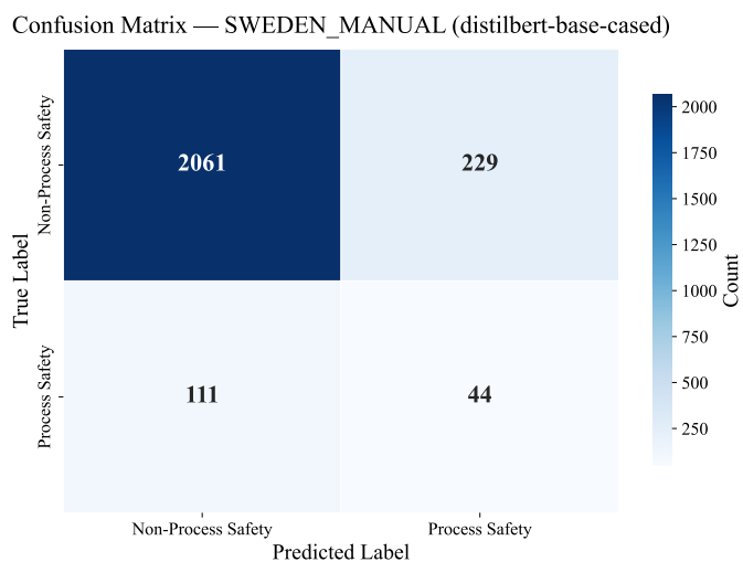
(c) distilbert-base-cased.
