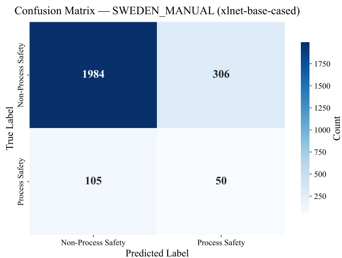
(f) xlnet-base-cased.
