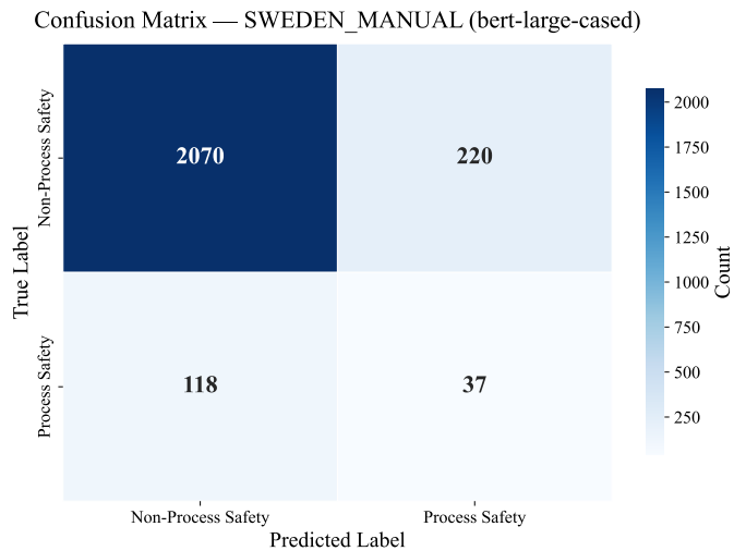
(b) bert-large-cased.
