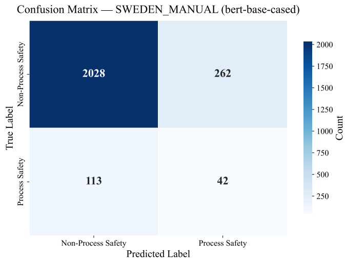
(a) bert-base-cased.
