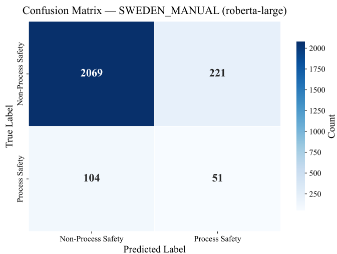
(e) roberta-large.
