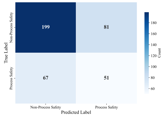
(b) bert-base-multilingual-uncased.
