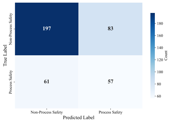
(a) bert-base-multilingual-cased.
