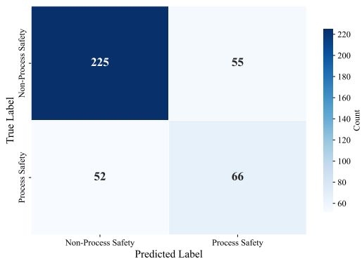
(e) intfloat_multilingual-e5-large-instruct.
