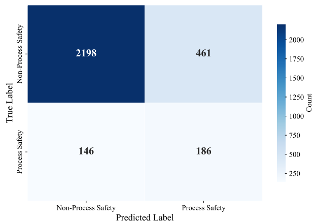
(a) bert-base-multilingual-cased.
