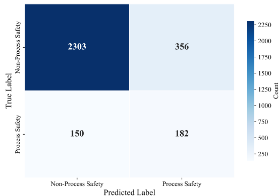
(e) intfloat_multilingual-e5-large-instruct.
