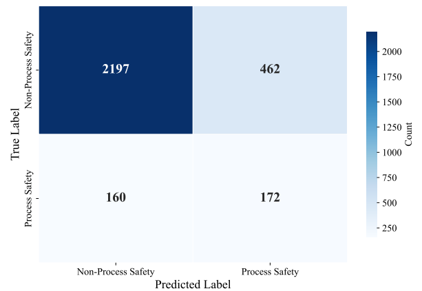
(b) bert-base-multilingual-uncased.
