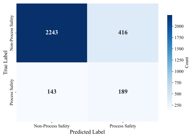
(c) intfloat_multilingual-e5-base.
