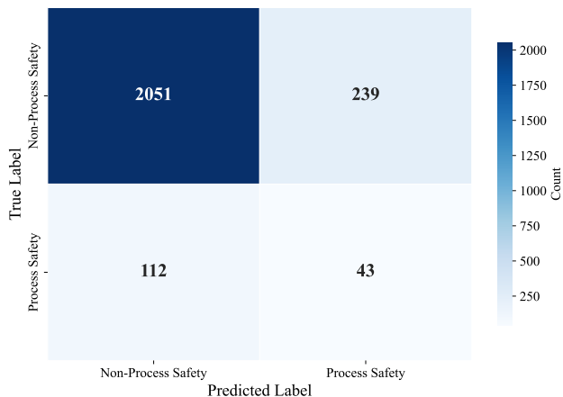
(c) intfloat_multilingual-e5-base.
