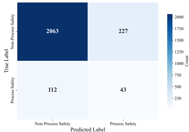
(b) bert-base-multilingual-uncased.
