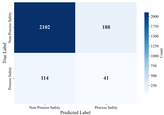
(e) intfloat_multilingual-e5-large-instruct.
