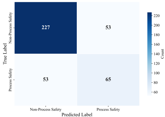
Confusion Matrix — DUTCH_MANUAL (intfloat/multilingual-e5-large-instruct, SVM)
