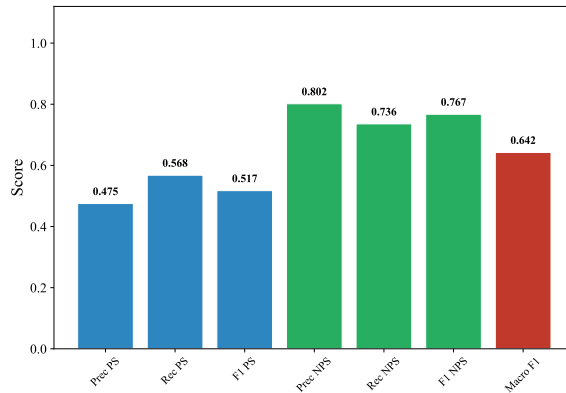
Classification Metrics — DUTCH_MANUAL (snowflake-arctic-embed-l-v2.0, SVM)
