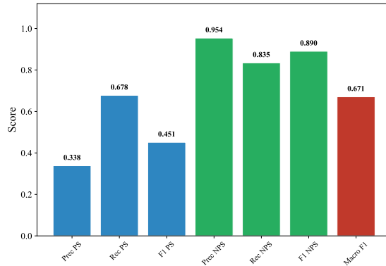
Classification Metrics — GERMAN_MANUAL (bert-base-multilingual-uncased, SVM)
