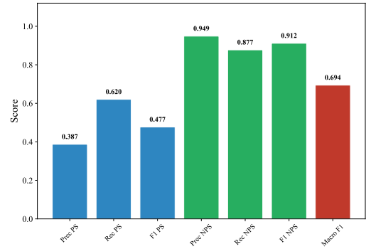
(b) Per-Class Metrics.
