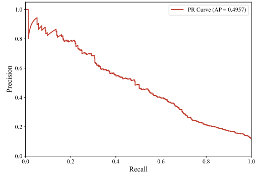
(c) Precision-Recall Curve.
