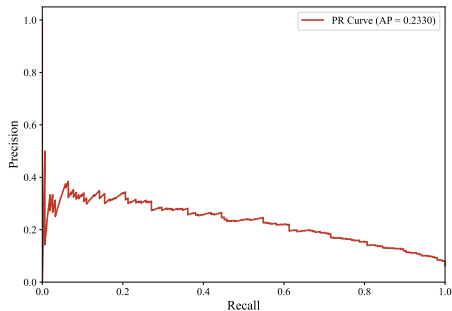
(c) Precision-Recall Curve.
