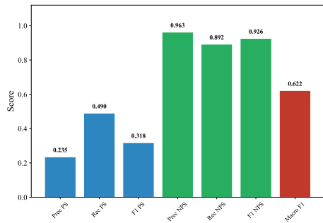
(b) Per-Class Metrics.
