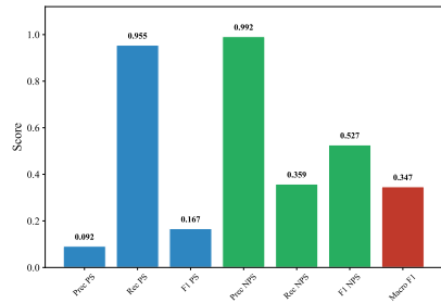
(b) Per-Class Metrics.
