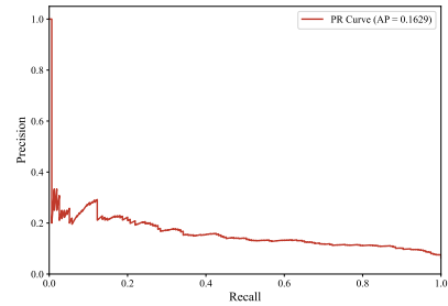
(c) Precision-Recall Curve.
