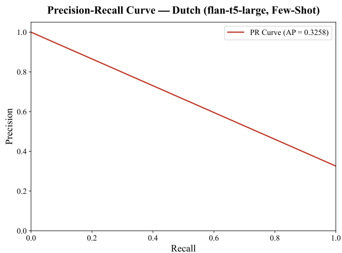
(c) Precision-Recall Curve.
