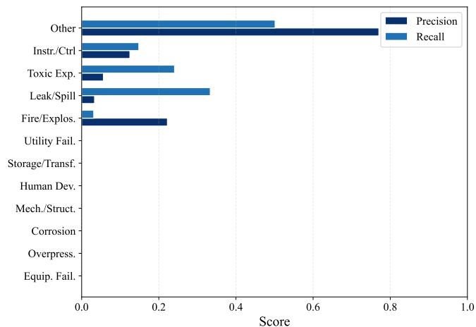
(c) precision vs recall.
