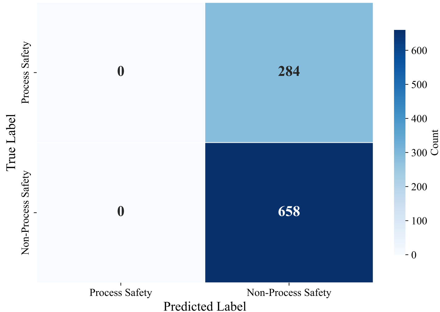
Confusion Matrix — English (flan-t5-large, Few-Shot)
