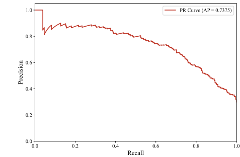
(c) Precision-Recall Curve.
