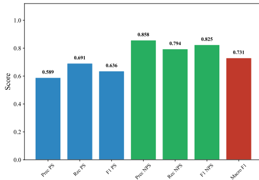
Classification Metrics — ENGLISH_MANUAL (intfloat/multilingual-e5-large-instruct, SVM)
