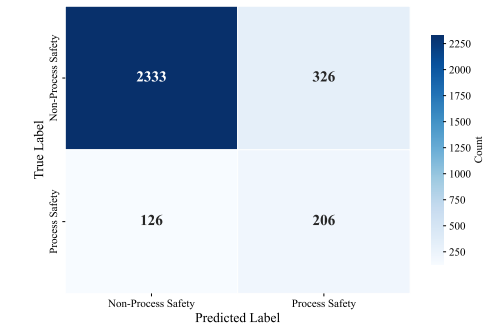
(a) Confusion Matrix.
