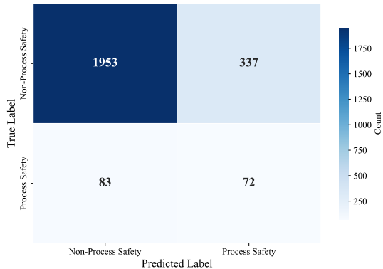
Confusion Matrix — SWEDISH_MANUAL (efederici/e5-base-multilingual-4096, SVM)
