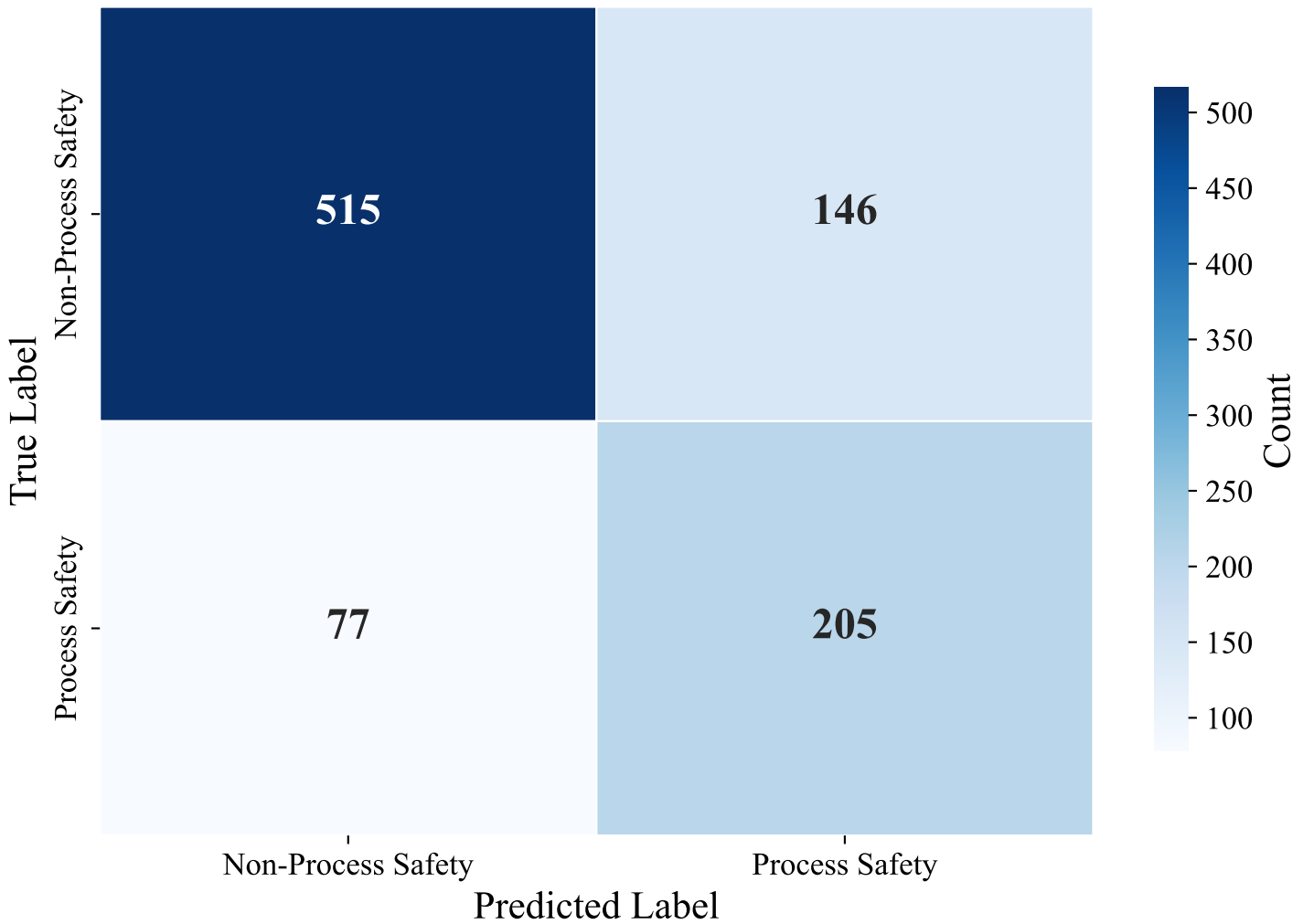
Confusion Matrix — ENGLISH_MANUAL (distilbert-base-cased)
