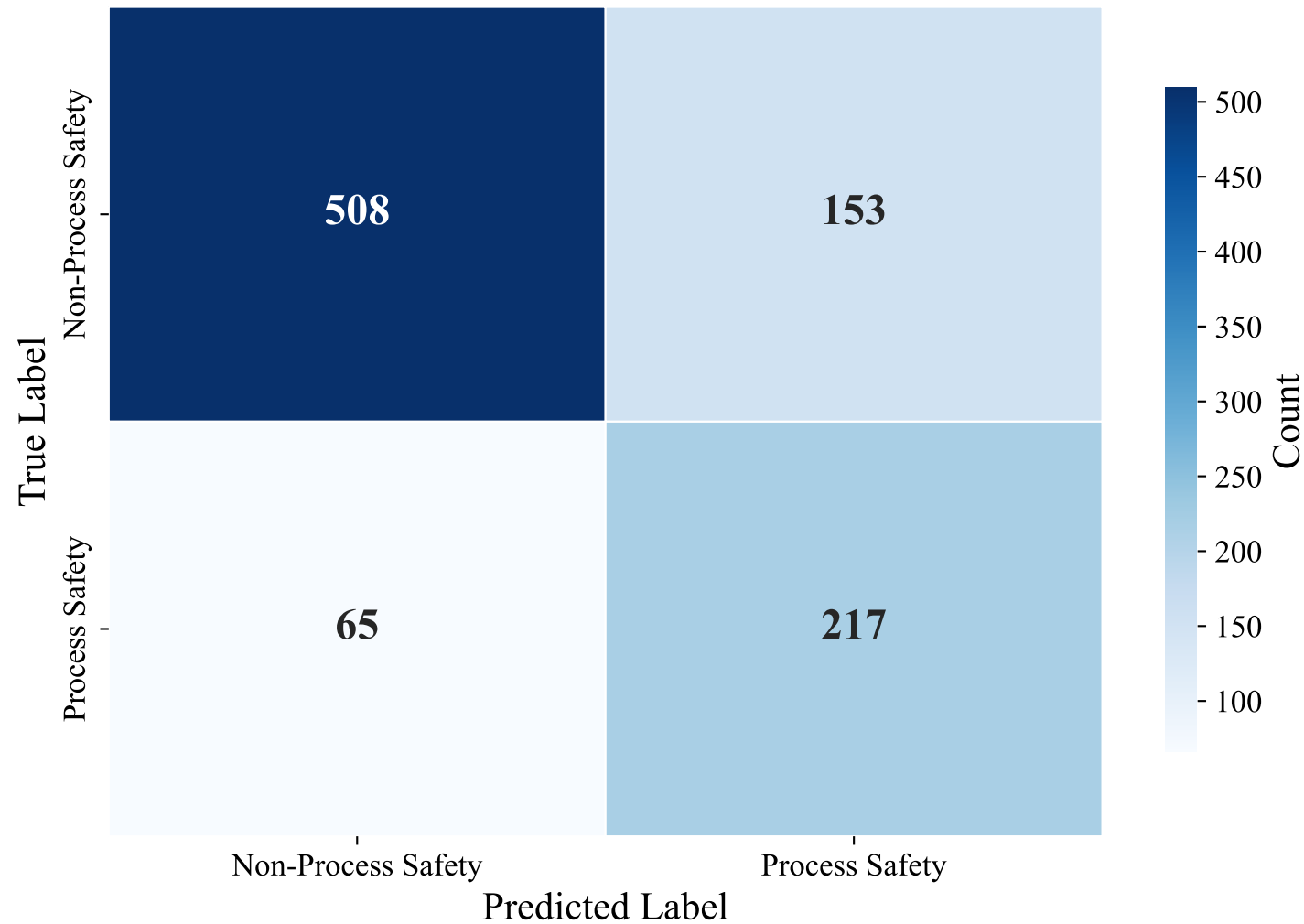
Confusion Matrix — ENGLISH_MANUAL (roberta-large)
