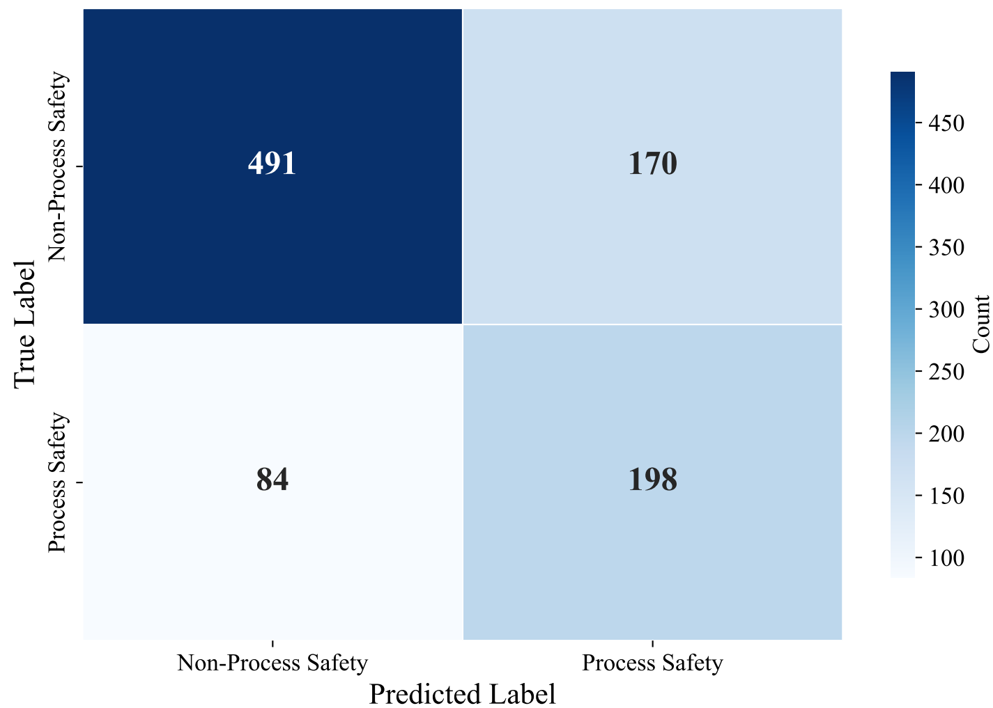
Confusion Matrix — ENGLISH_MANUAL (bert-base-multilingual-uncased)
