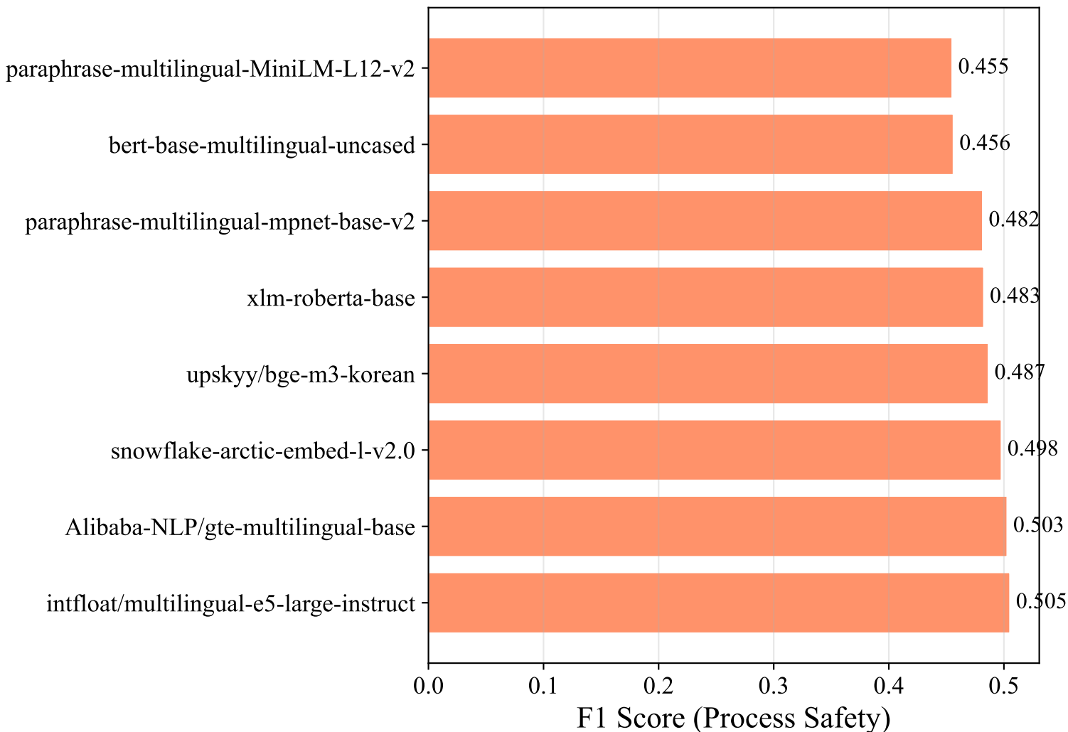
Average F1 Score by Model — Iteration 4
