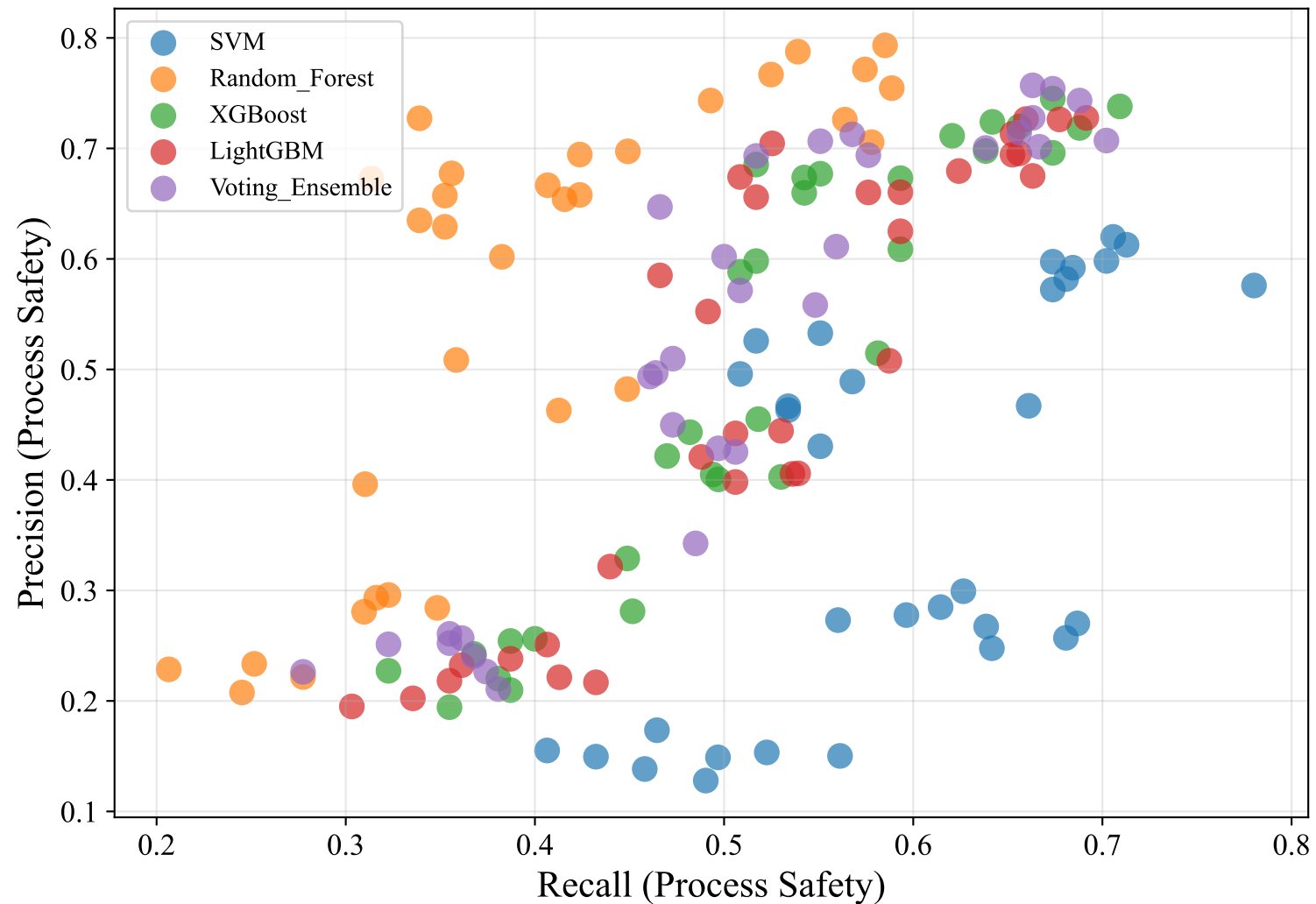
Precision vs Recall (PS) by Classifier — Iteration 4
