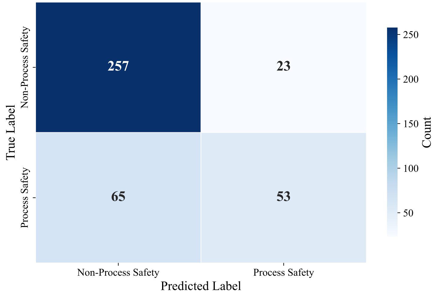
Confusion Matrix — DUTCH_MANUAL (Alibaba-NLP/gte-multilingual-base, Random_Forest)
