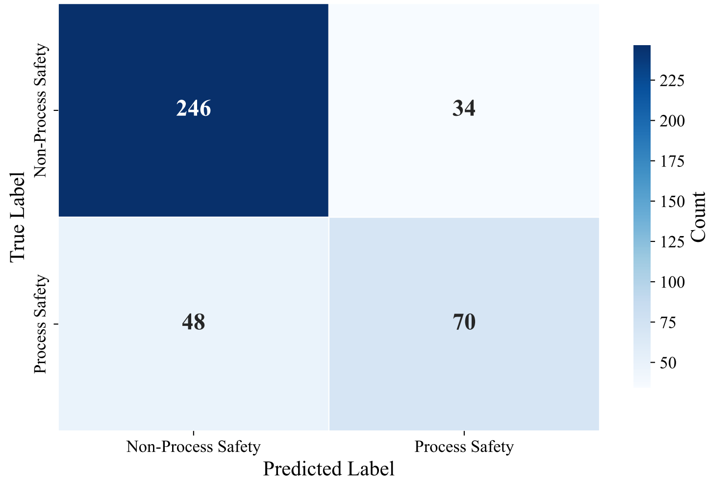
Confusion Matrix — DUTCH_MANUAL (Alibaba-NLP/gte-multilingual-base, XGBoost)
