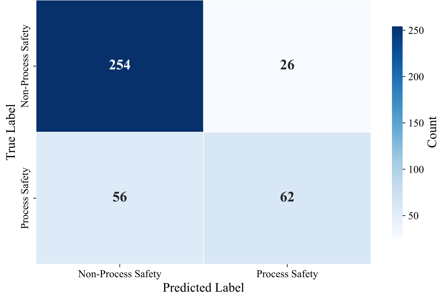
Confusion Matrix — DUTCH_MANUAL (snowflake-arctic-embed-l-v2.0, LightGBM)
