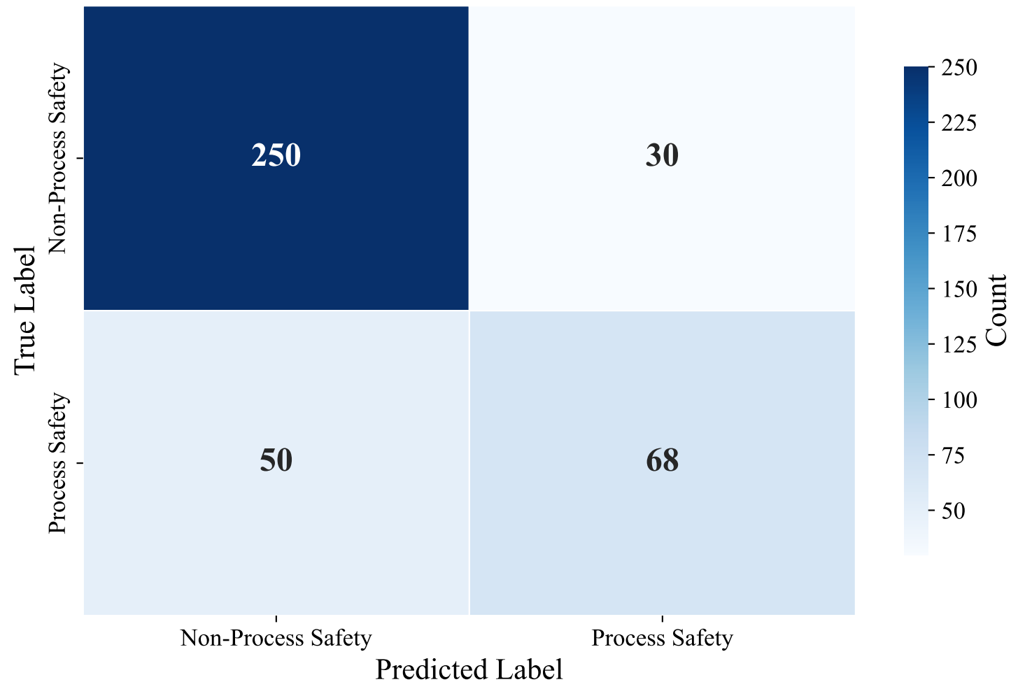
Confusion Matrix — DUTCH_MANUAL (upskyy/bge-m3-korean, Voting_Ensemble)
