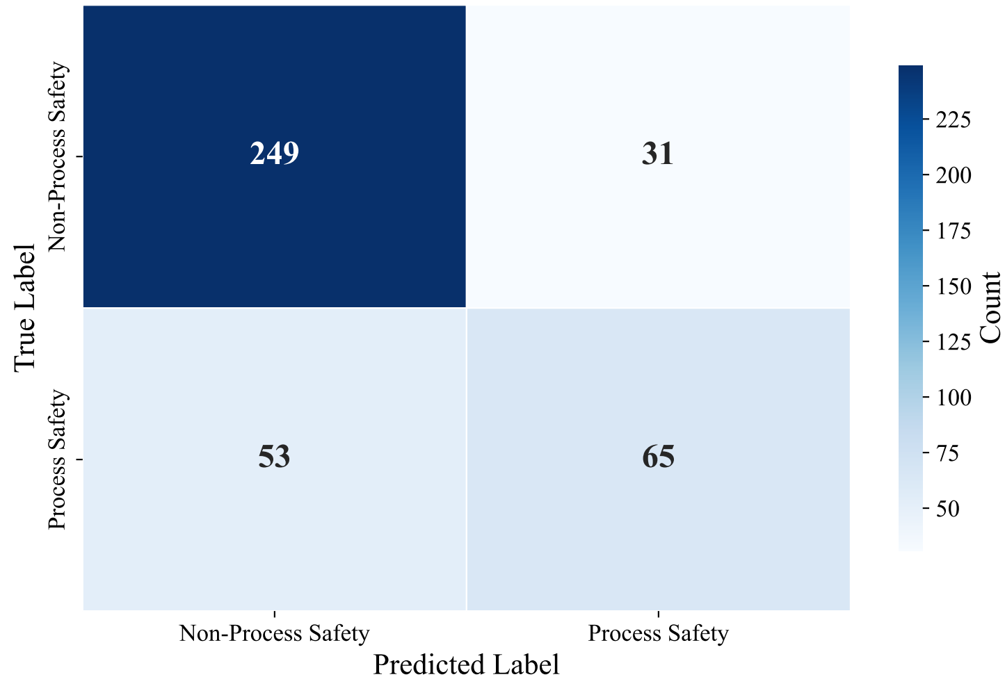
Confusion Matrix — DUTCH_MANUAL (upskyy/bge-m3-korean, XGBoost)
