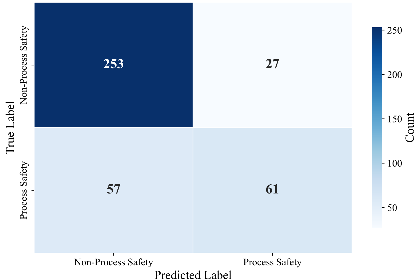
Confusion Matrix — DUTCH_MANUAL (xlm-roberta-base, Voting_Ensemble)
