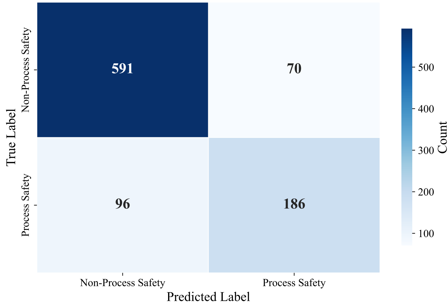
Confusion Matrix — ENGLISH_MANUAL (Alibaba-NLP/gte-multilingual-base, LightGBM)
