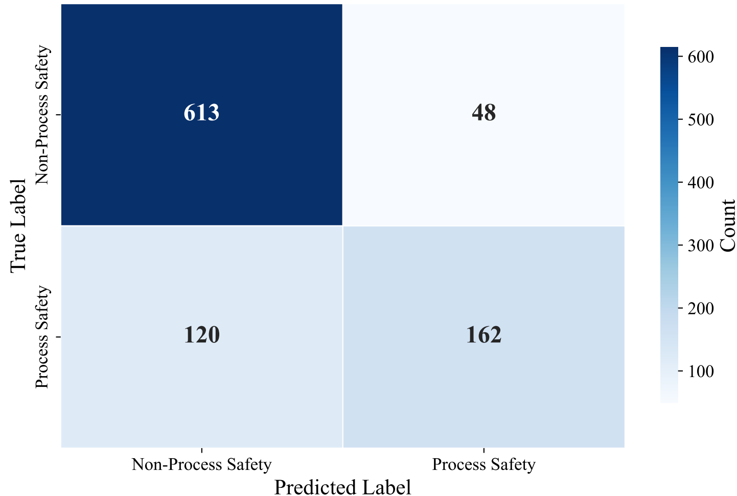
Confusion Matrix — ENGLISH_MANUAL (Alibaba-NLP/gte-multilingual-base, Random_Forest)
