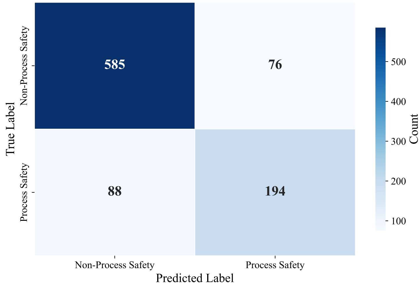
Confusion Matrix — ENGLISH_MANUAL (intfloat/multilingual-e5-large-instruct, XGBoost)
