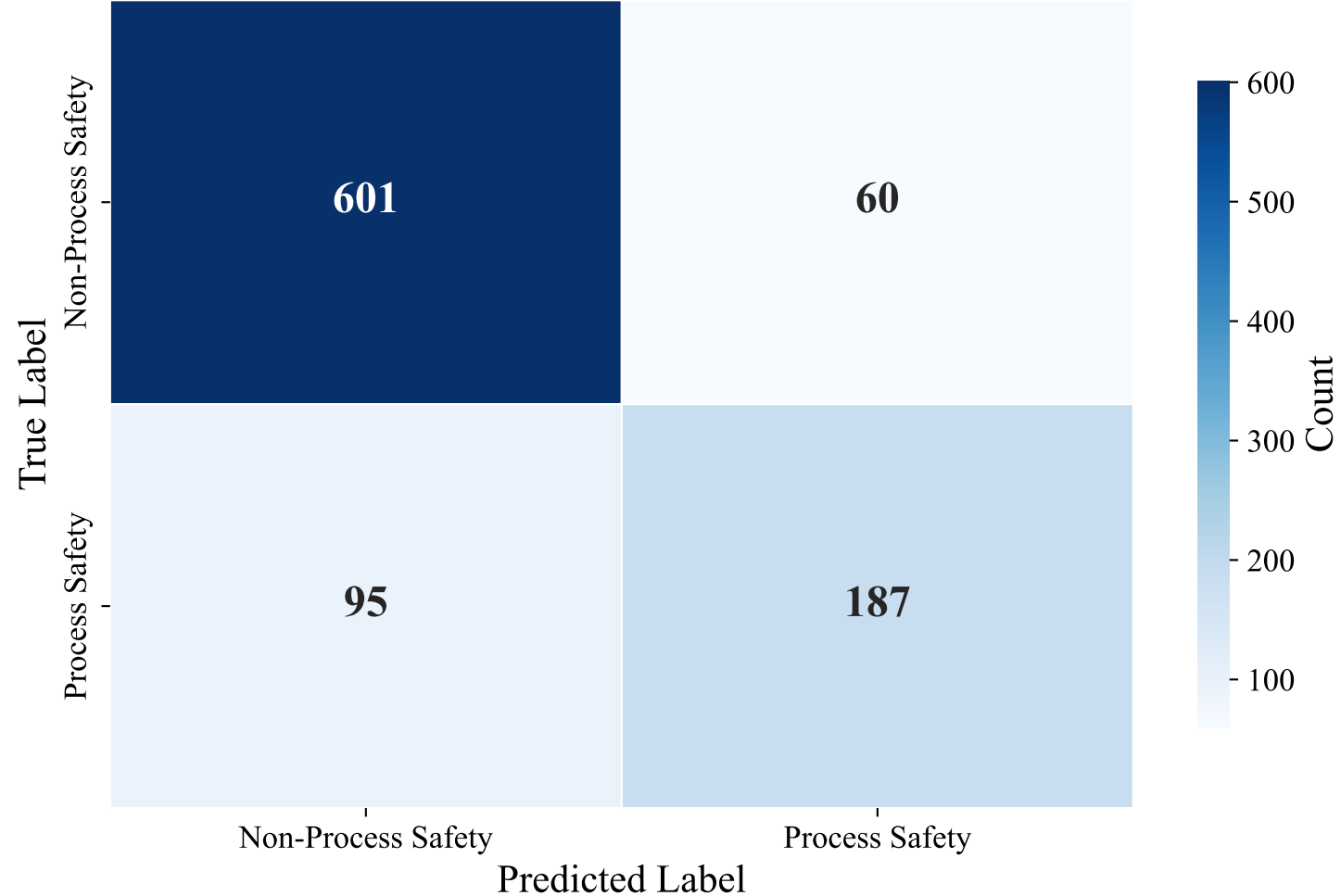
Confusion Matrix — ENGLISH_MANUAL (snowflake-arctic-embed-l-v2.0, Voting_Ensemble)
