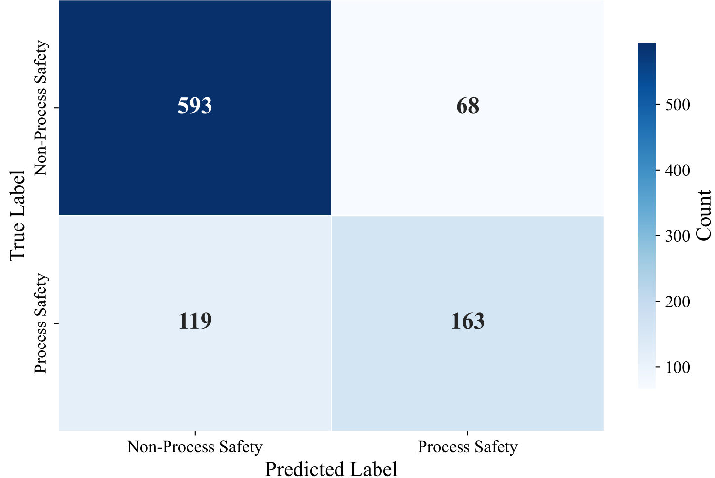
Confusion Matrix — ENGLISH_MANUAL (xlm-roberta-base, Random_Forest)
