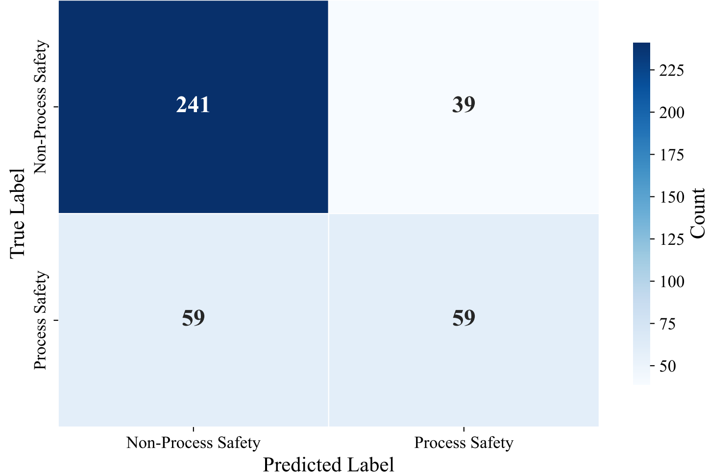
Confusion Matrix — NETHERLANDS_MANUAL (bert-base-multilingual-uncased, Voting_Ensemble)
