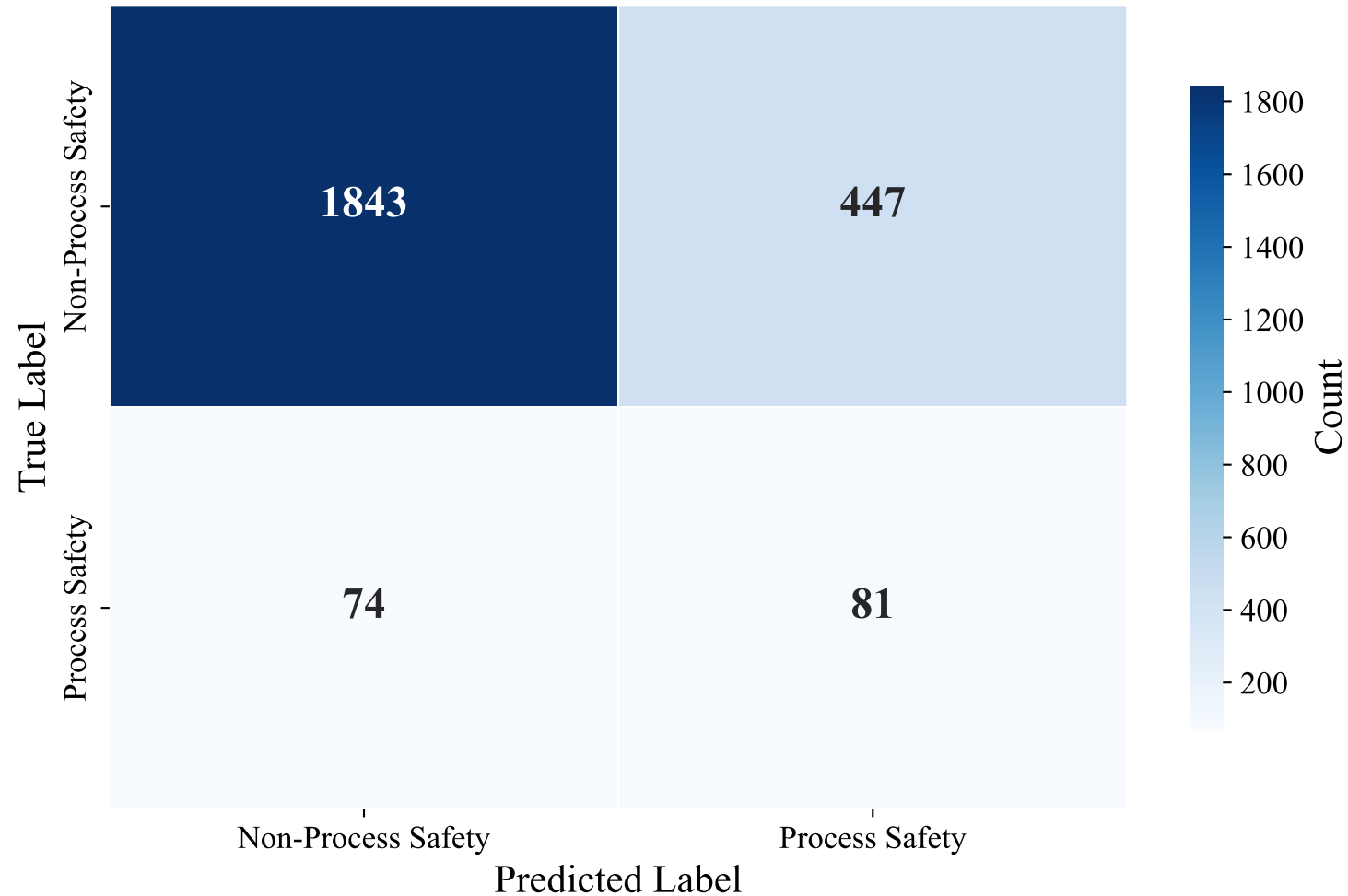
Confusion Matrix — SWEDISH_MANUAL (paraphrase-multilingual-mpnet-base-v2, SVM)
