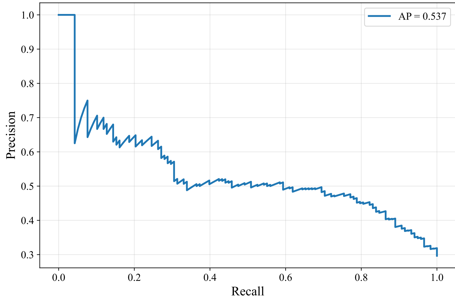
Precision-Recall Curve — DUTCH_MANUAL (intfloat/multilingual-e5-large-instruct, SVM)
