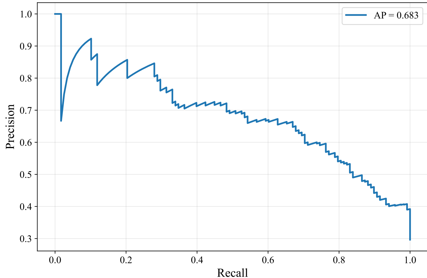
Precision-Recall Curve — DUTCH_MANUAL (intfloat/multilingual-e5-large-instruct, XGBoost)
