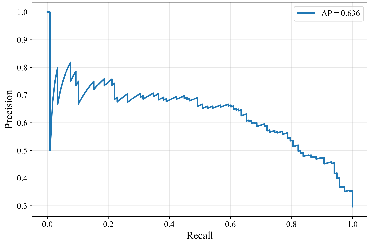
Precision-Recall Curve — DUTCH_MANUAL (upskyy/bge-m3-korean, LightGBM)
