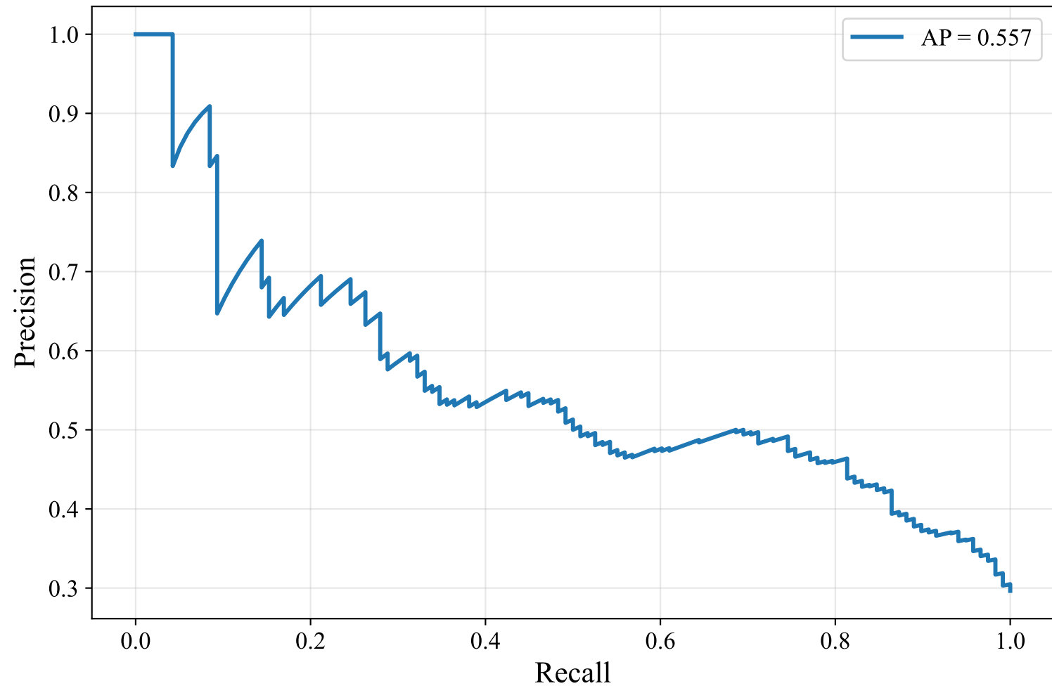
Precision-Recall Curve — DUTCH_MANUAL (upskyy/bge-m3-korean, SVM)
