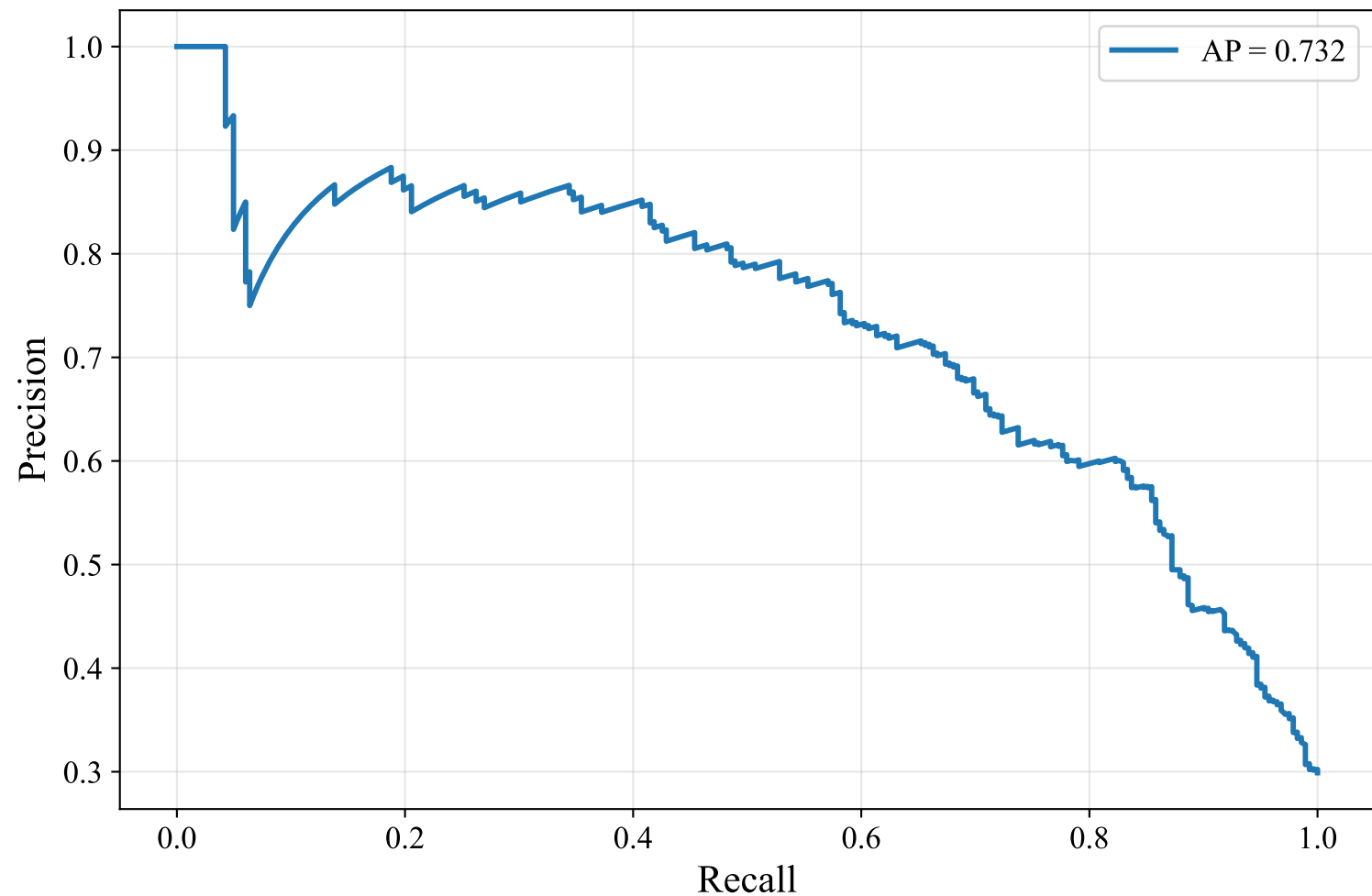
Precision-Recall Curve — ENGLISH_MANUAL (Alibaba-NLP/gte-multilingual-base, Random_Forest)
