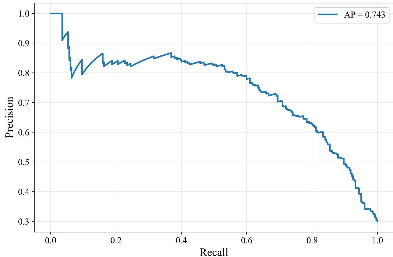
Precision-Recall Curve — ENGLISH_MANUAL (intfloat/multilingual-e5-large-instruct, Random_Forest)
