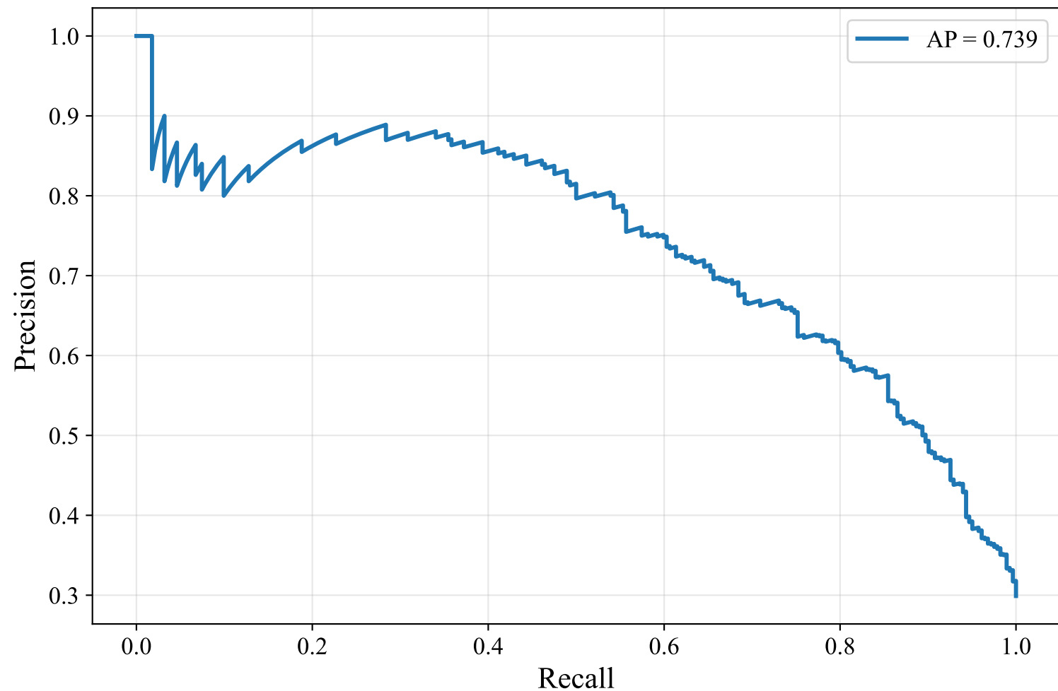
Precision-Recall Curve — ENGLISH_MANUAL (paraphrase-multilingual-mpnet-base-v2, LightGBM)
