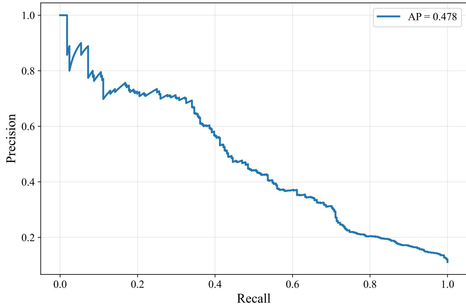
Precision-Recall Curve — GERMAN_MANUAL (Alibaba-NLP/gte-multilingual-base, Random_Forest)
