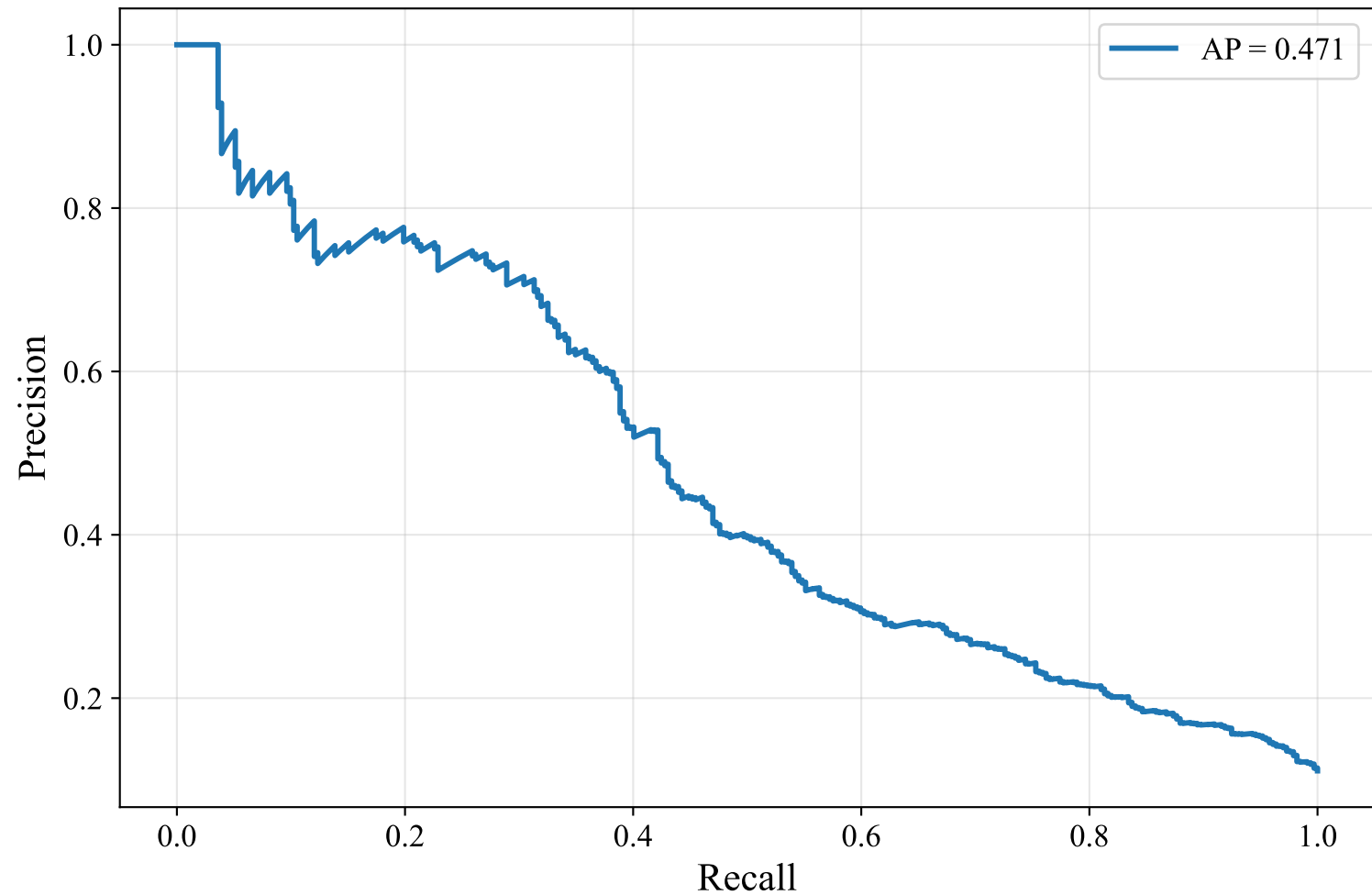
Precision-Recall Curve — GERMAN_MANUAL (Alibaba-NLP/gte-multilingual-base, XGBoost)
